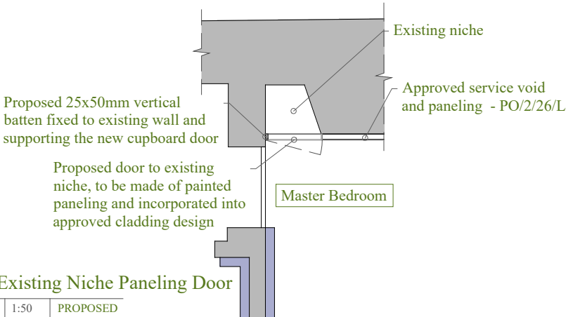
E1 1:50 PROPOSED
