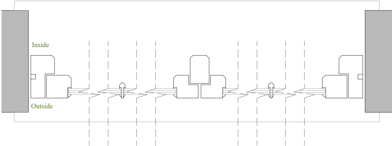
New Window - Plan
