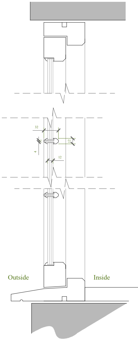
New Window - Section
