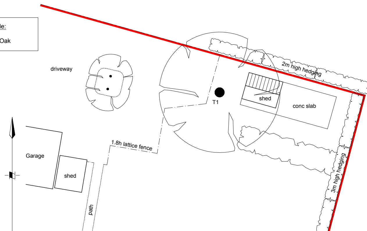
Existing Site plan 1:200 @ A3
