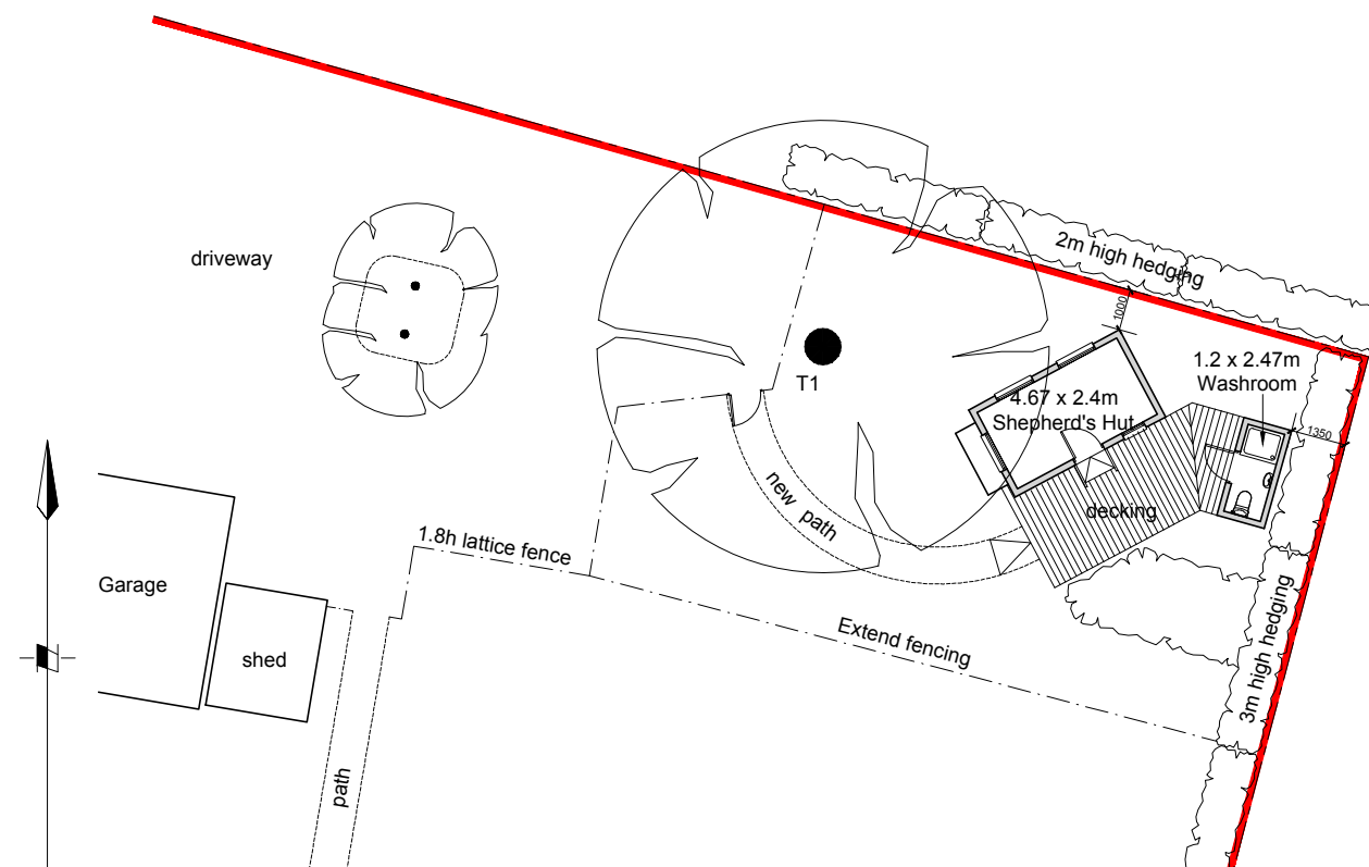
Proposed Site plan 1:200 @ A3
