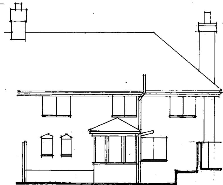
SOUTH EXISTING ELEVATIONS
