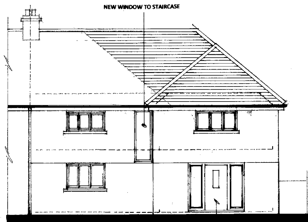
NORTH ELEVATION TO ARUNDEL ROAD
