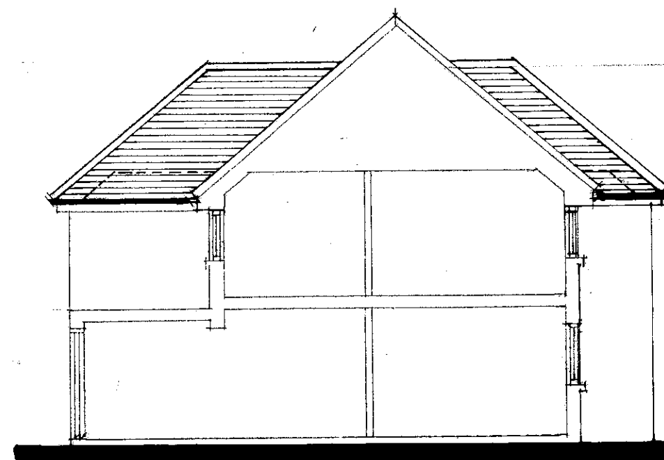
EAST ELEVATION / SECTION
