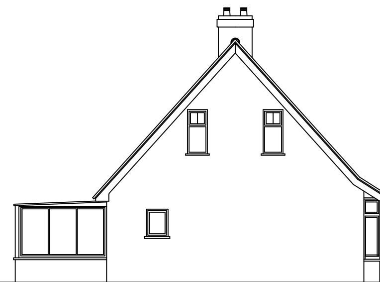
Existing North N/East Elevation
