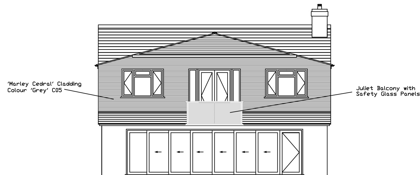
Proposed South E/East Elevation
