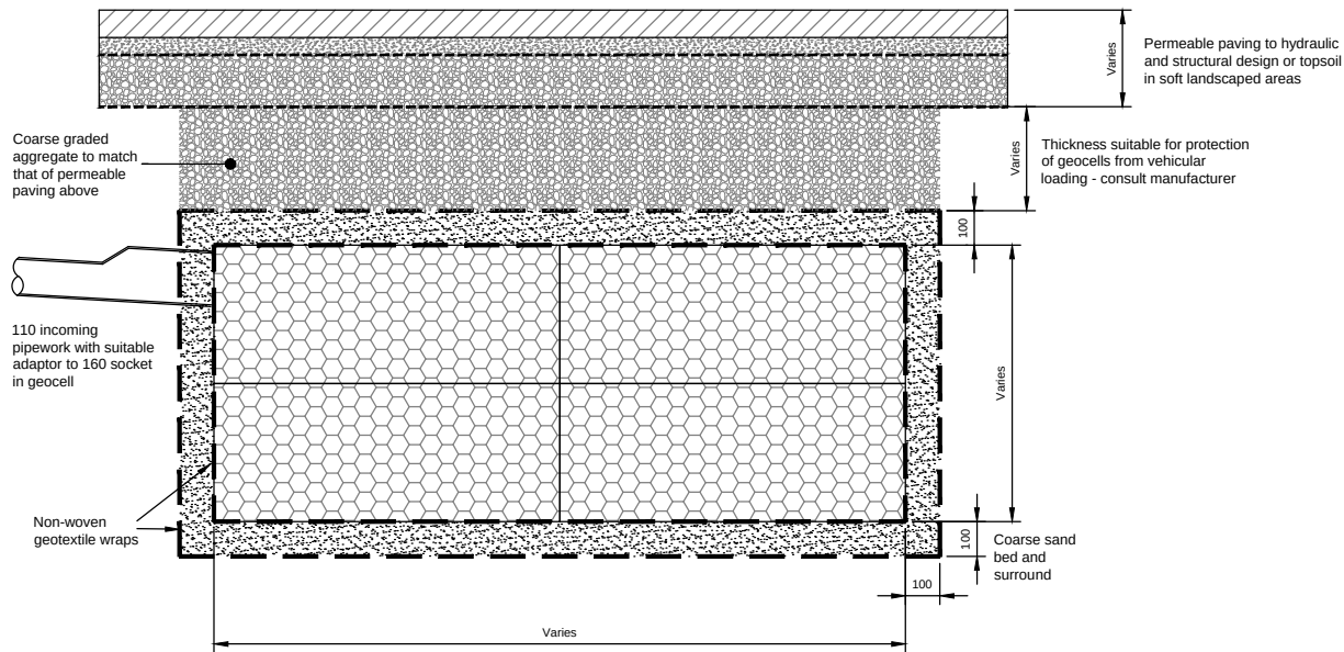
Typical Geocellular soakaway Unit (for use in permeable paved areas)
