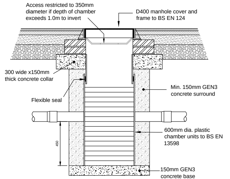
Typical Silt Trap Inspection Chamber Detail (for use in areas subject to traffic loading)
