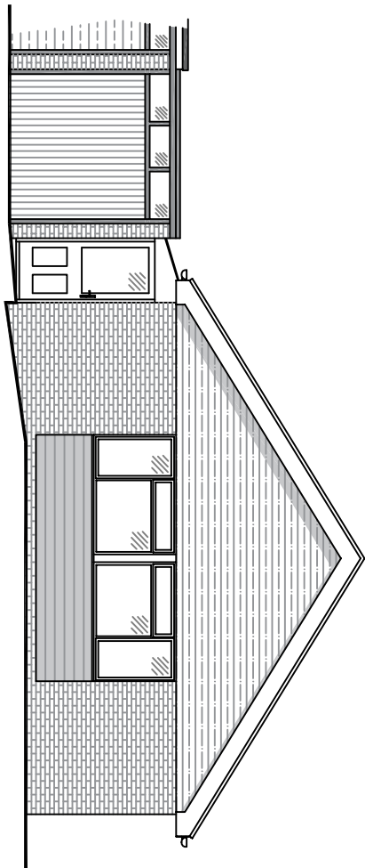
Existing Front (East) Elevation (Scale 1:100)
