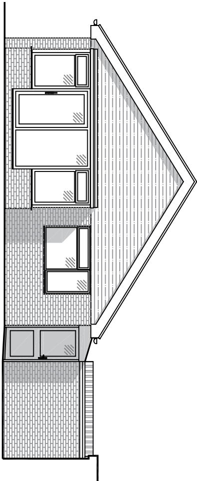
Existing Rear (West) Elevation (Scale 1:100)
