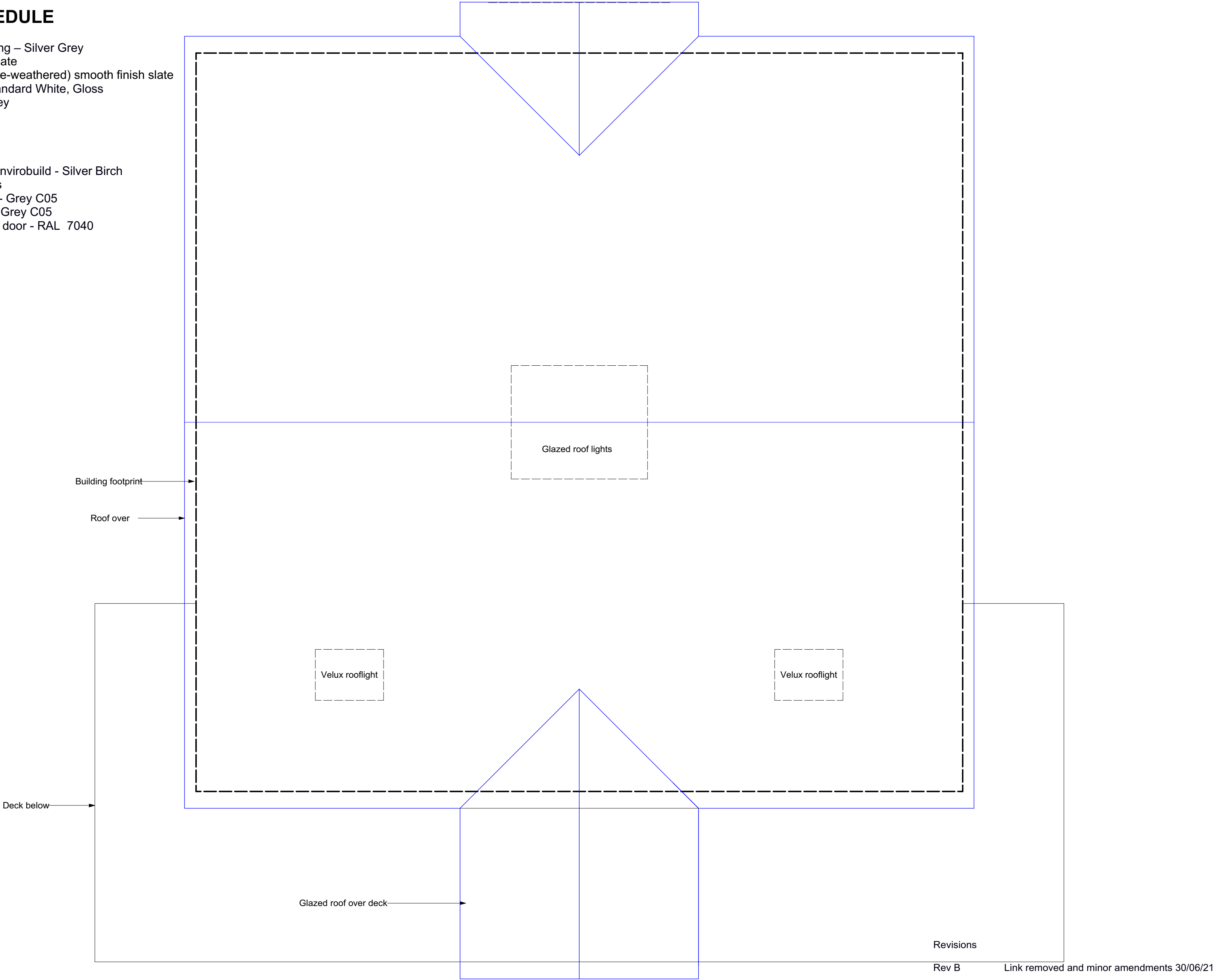
Roof Plan
