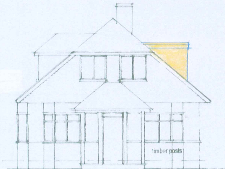
EAST ELEVATION
