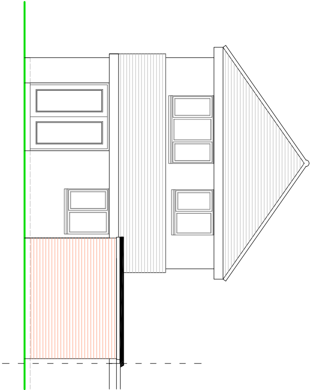
REAR ELEVATION
