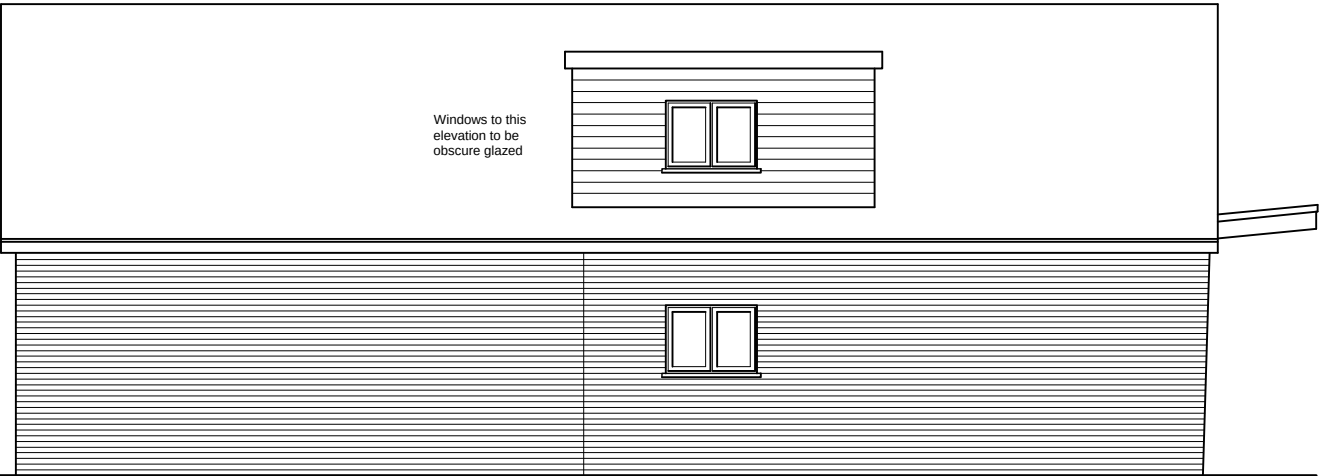
EAST ELEVATION
