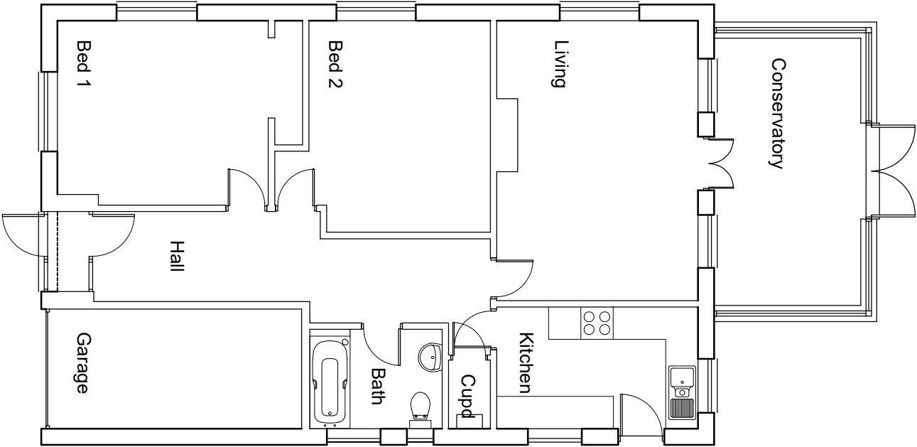
Floor Plan
