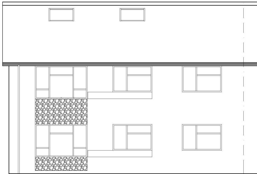
EXISTING SOUTH ELEVATION 1/100
