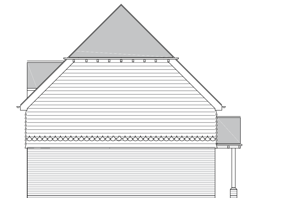
proposed side/south elevation
