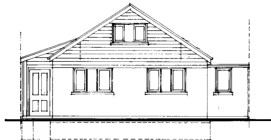
EAST ELEVATION TO SEA WAY
