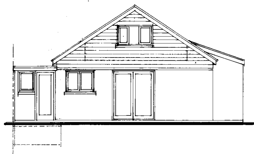
WEST ELEVATION TO REAR GARDEN
