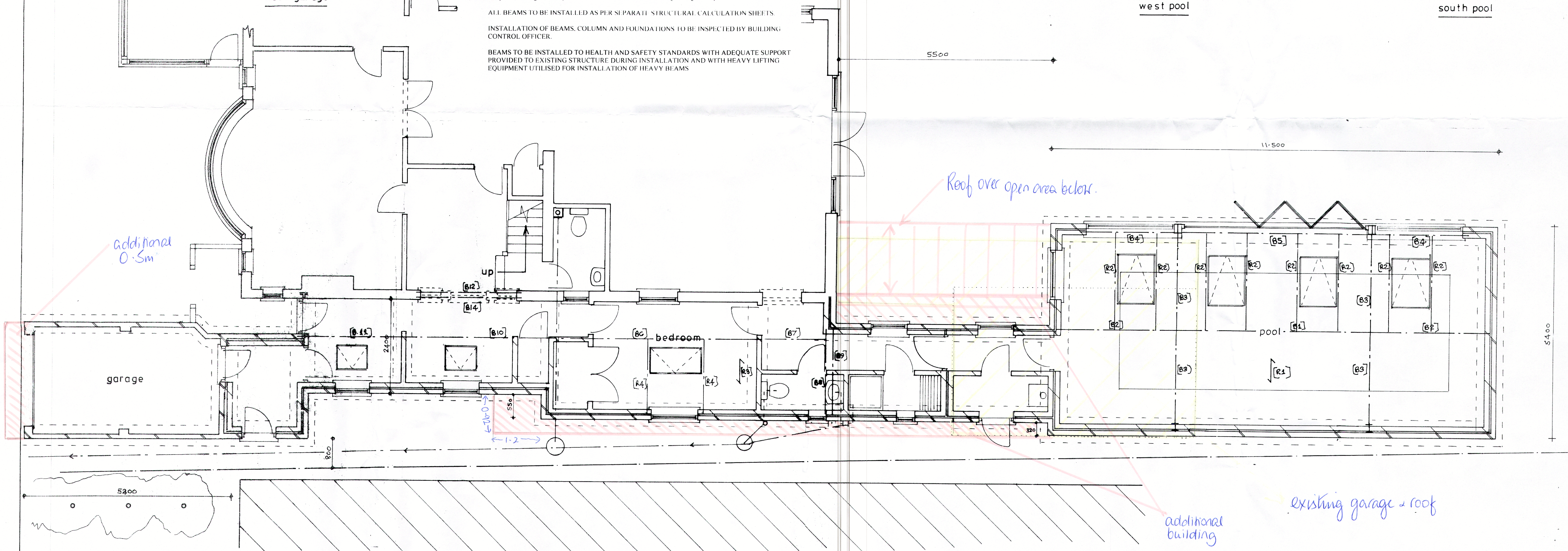
west garage
