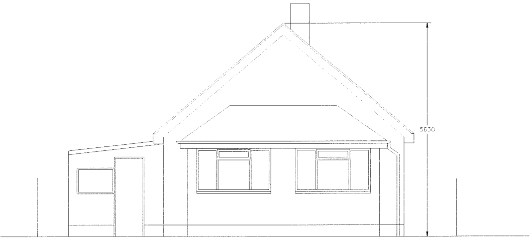
ELEVATION FACING SOUTH
