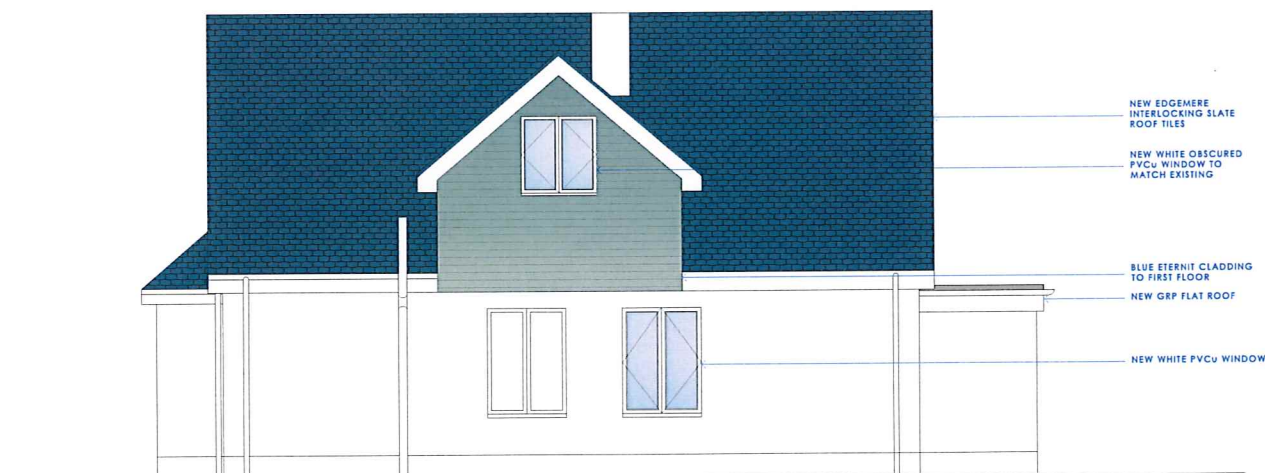
ELEVATION FACING EAST
