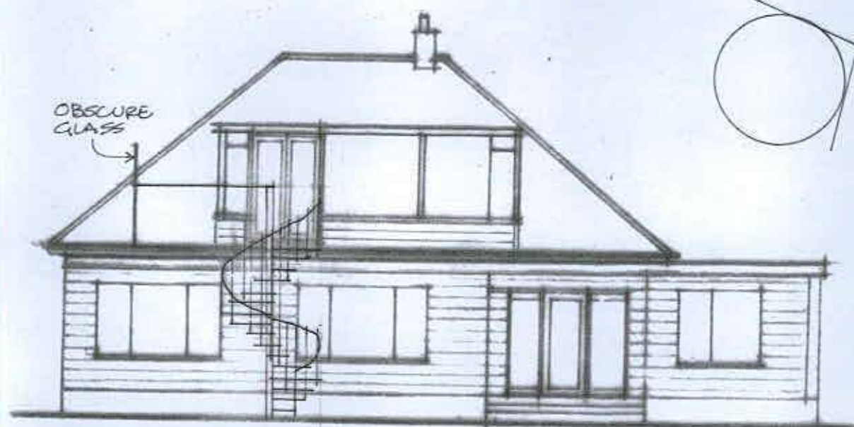
FRONT ELEVATION - EAST 1:100
