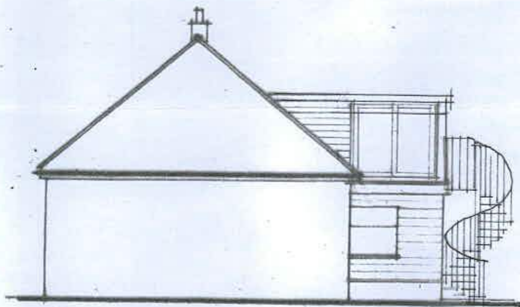
SIDE ELEVATION - SOUTH 1:100
