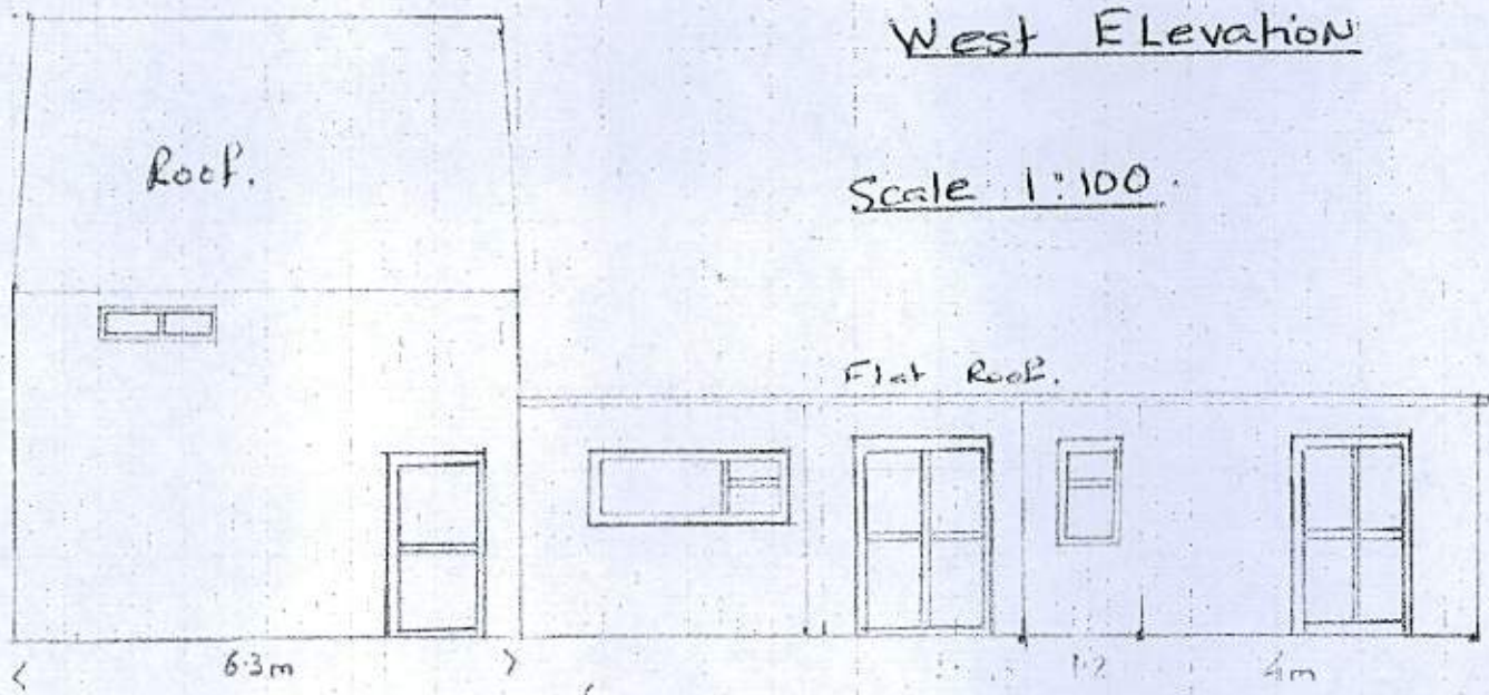
West proposed elevation
