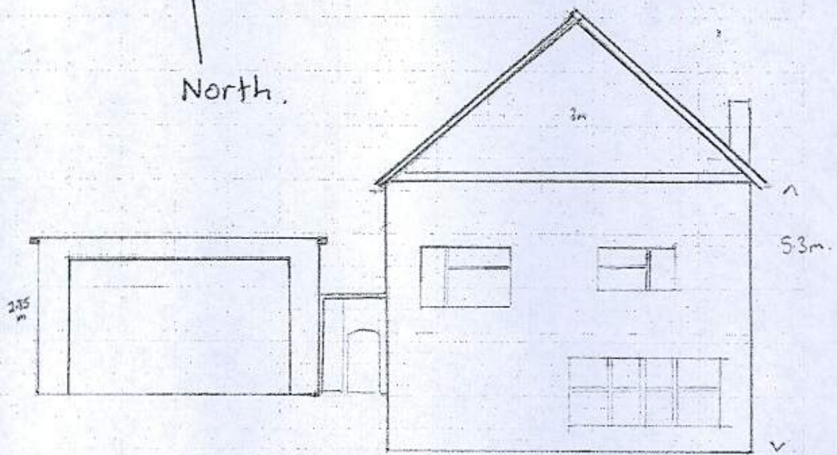
Existing (North) Front Elevation Scale 1:100.
