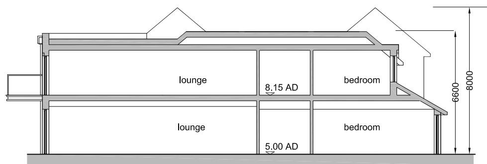
SECTION G-G
