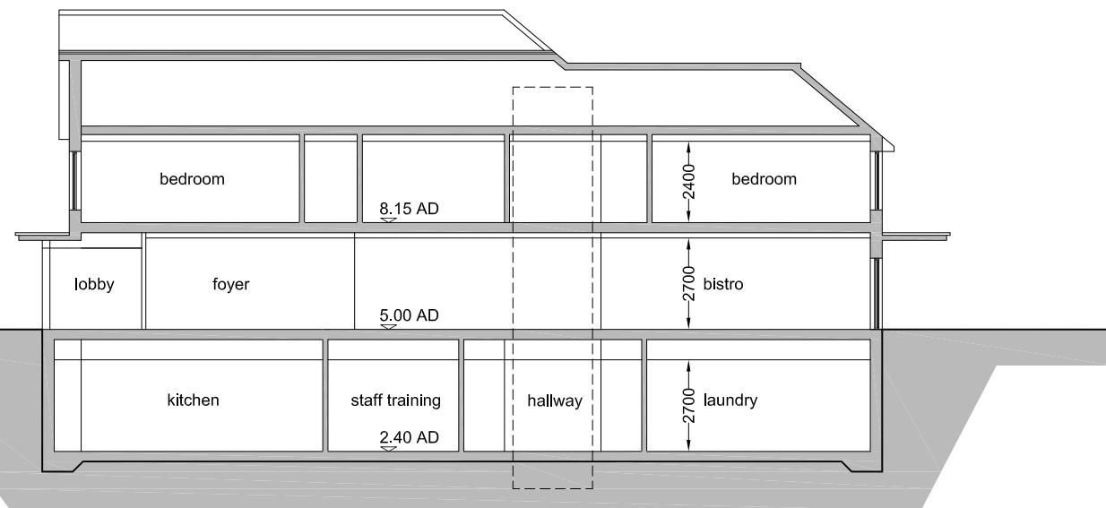
SECTION H-H
