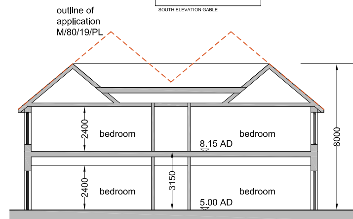
SECTION F-F
