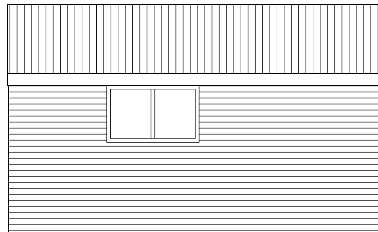
WEST ELEVATION
