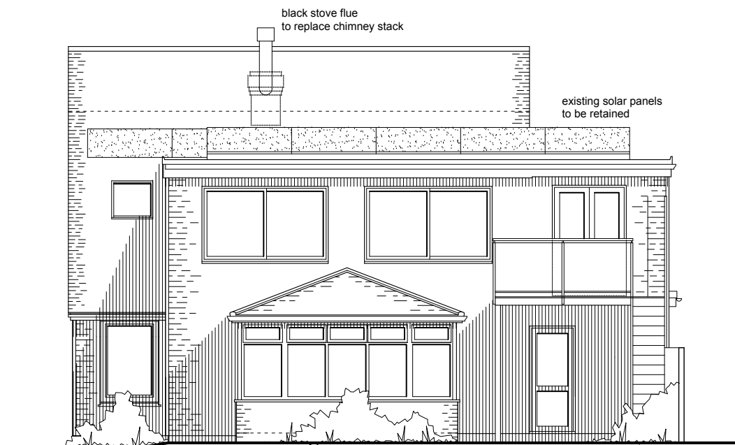
South Elevation
