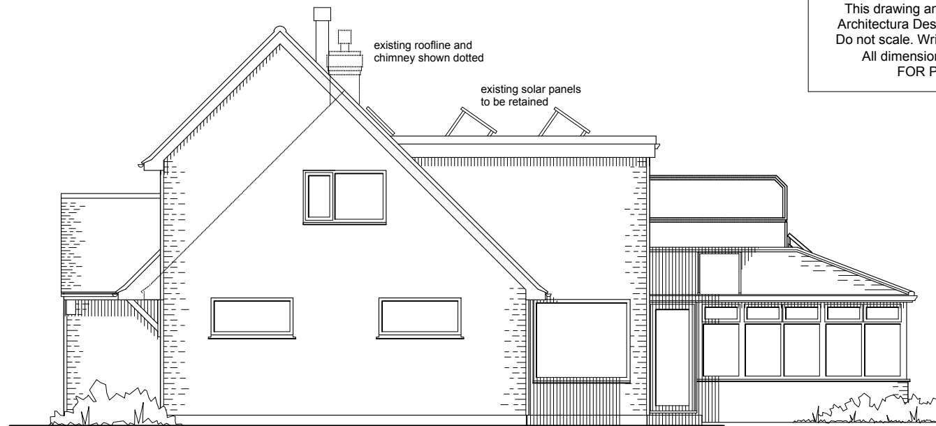
West Elevation
