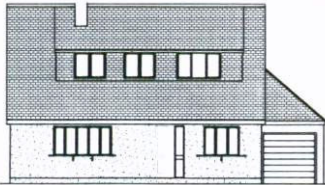
NEW WEST ELEVATION
