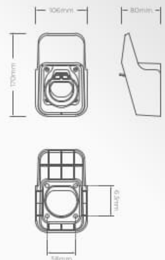
Type 2 charge gun holster:
