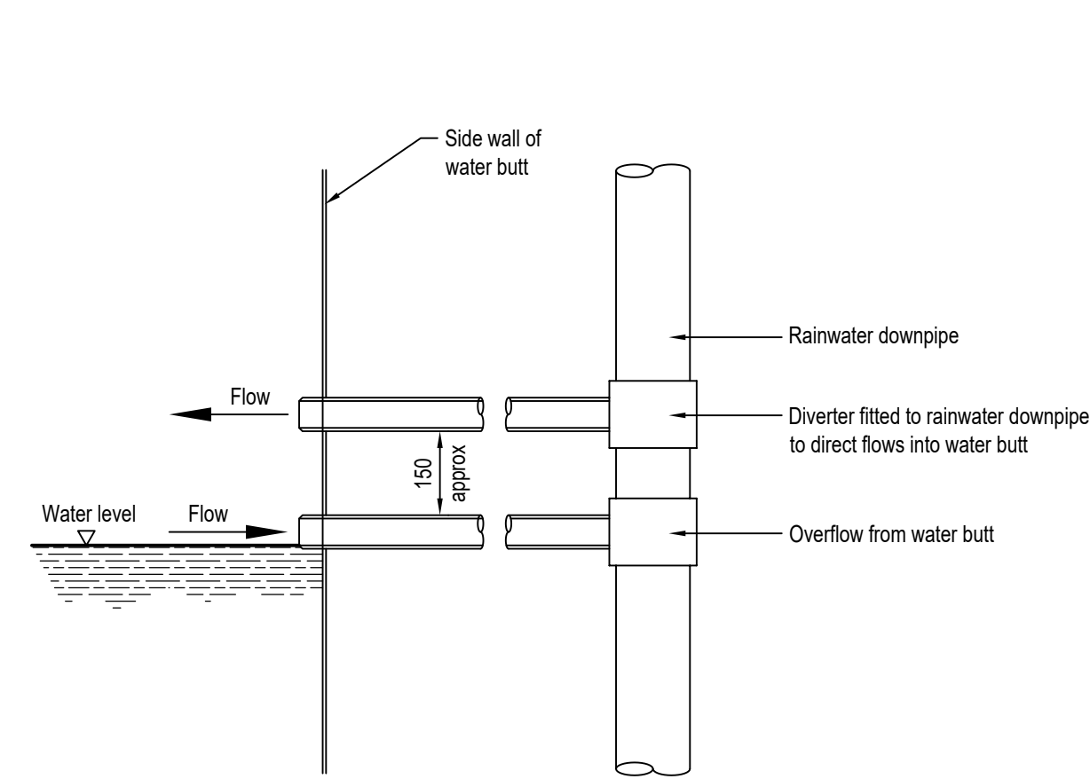
TYPICAL SECTION THROUGH RAINWATER DIVERTER
