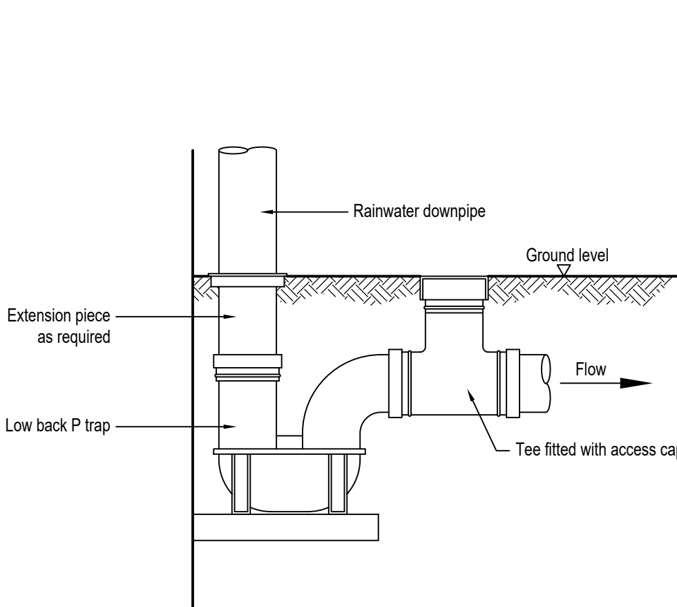
TYPICAL DETAIL AT BASE OF RAINWATER DOWNPIPES
