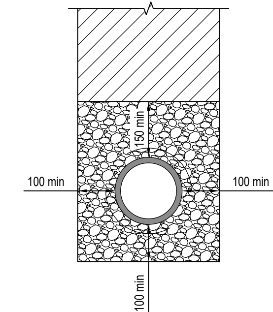
PIPE BEDDING FOR FLEXIBLE PIPES WITH MORE THAN 0.9m COVER BENEATH DRIVEWAYS AND VEHICULAR ACCESSES (Scale 1:10)
