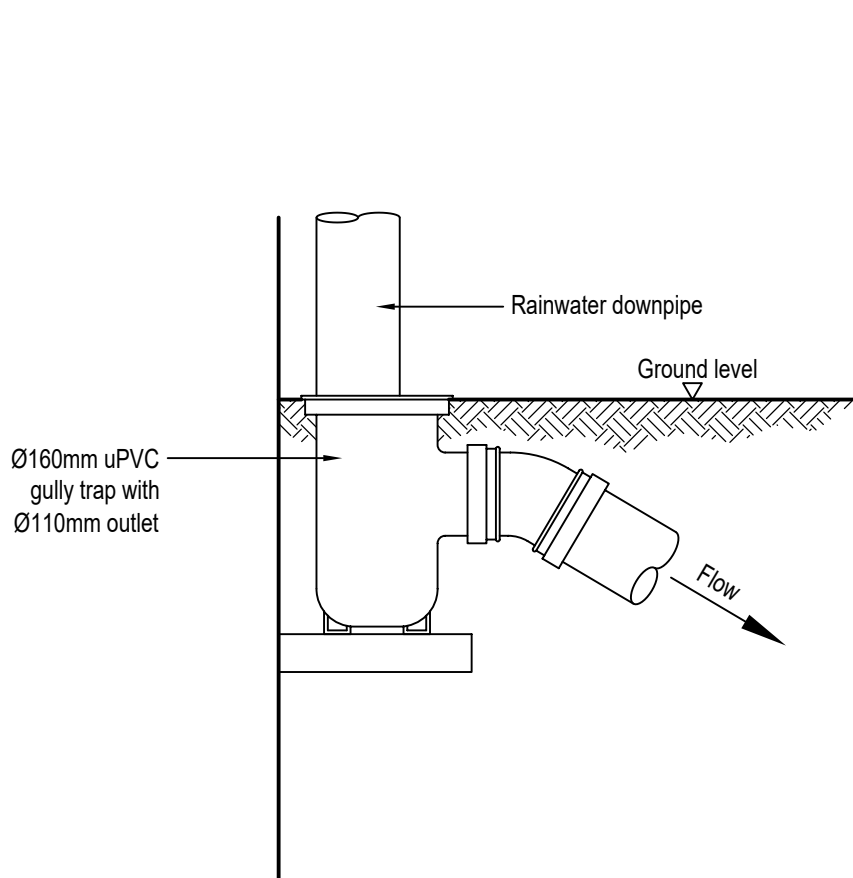
TYPICAL DETAIL AT BASE OF RAINWATER DOWNPIPES
