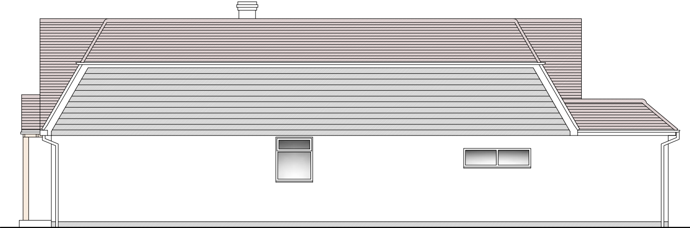
Proposed North Elevation (side) 1:100 @ A3
