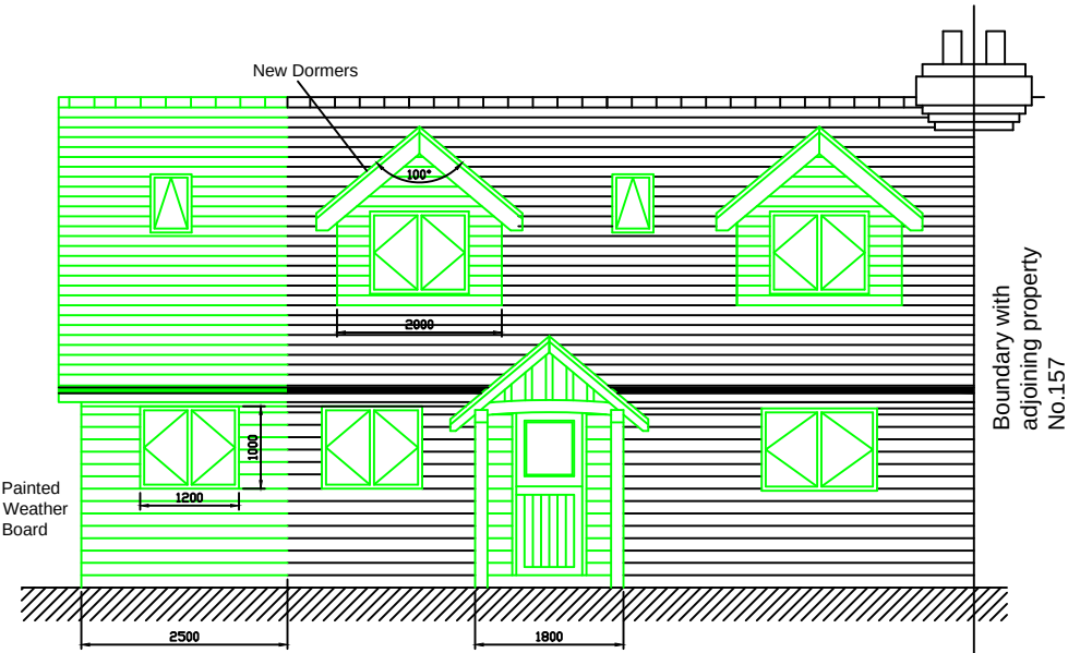
North Facing - Front Elevation to Entrance Drive
