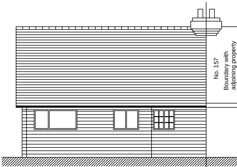
North Facing - Front Elevation To Entrance Drive
