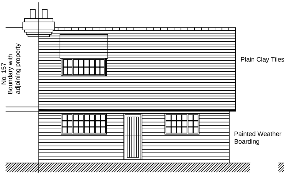
South Facing - Rear Elevation To Garden
