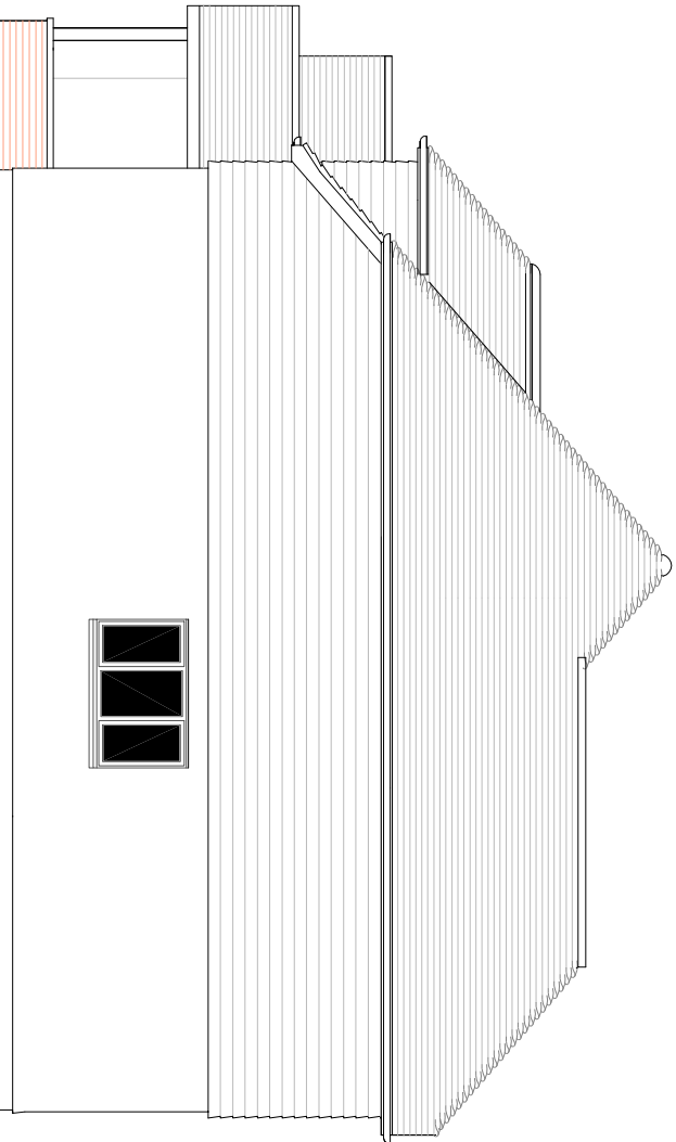
SIDE ELEVATION
