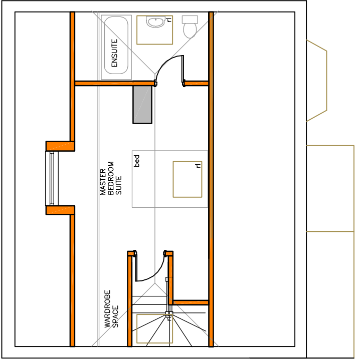
PROPOSED SECOND FLOOR PLAN 1:100
