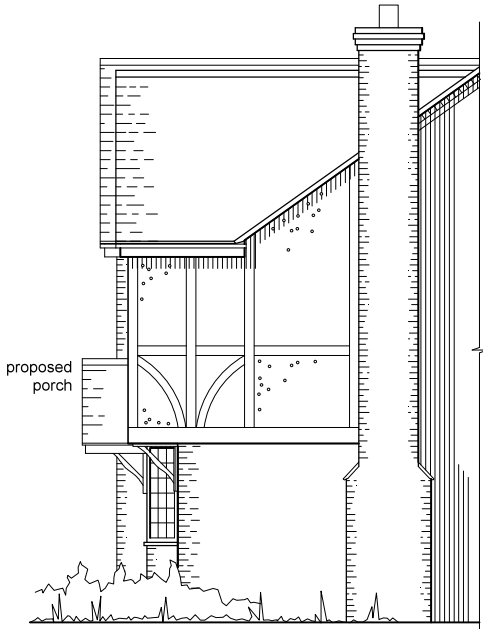
West Elevation
