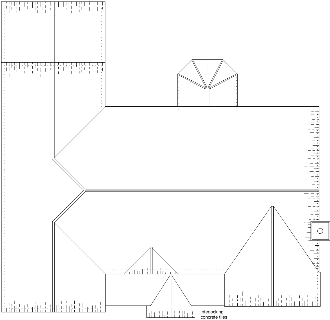
Roof Plan
