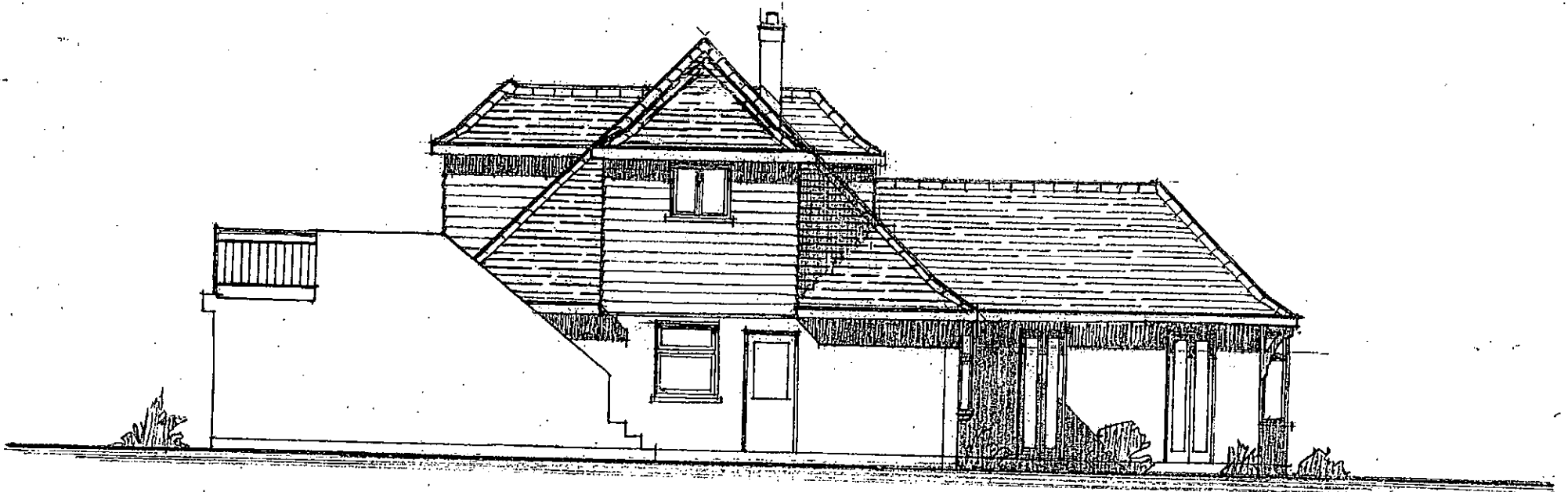
East elevation
