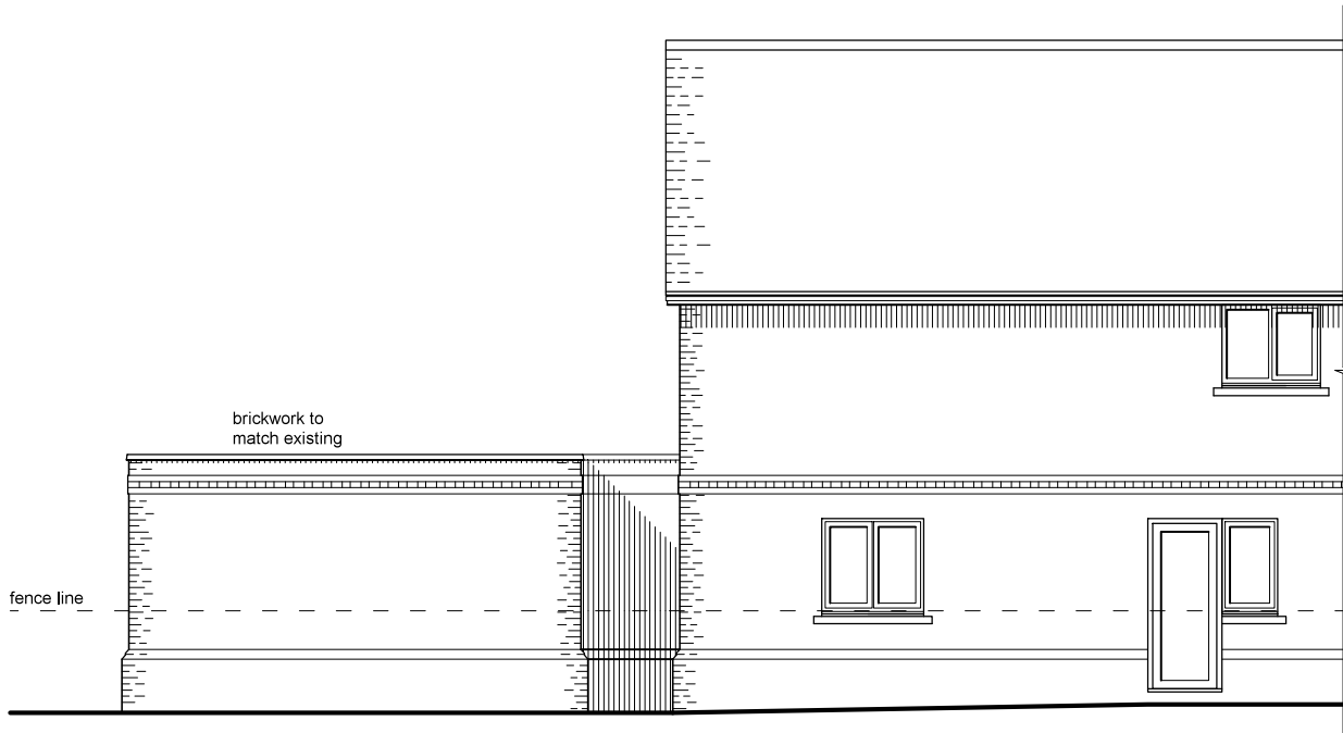
West Elevation
