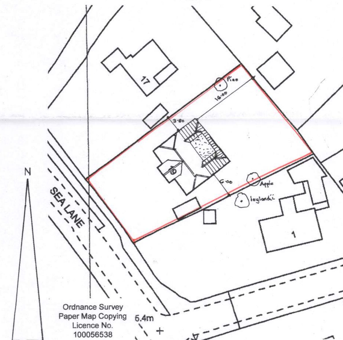
block plan
