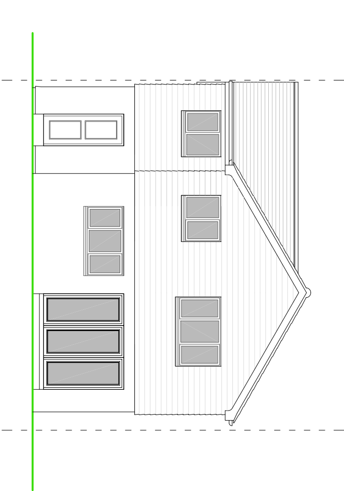
REAR ELEVATION
