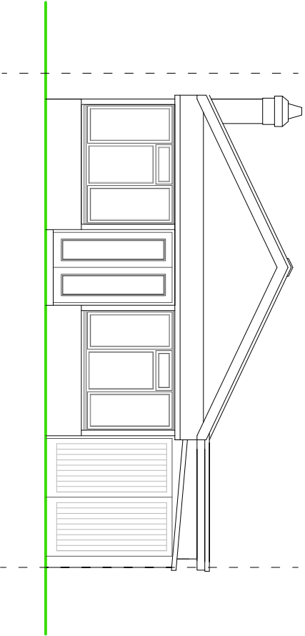
FRONT ELEVATION
