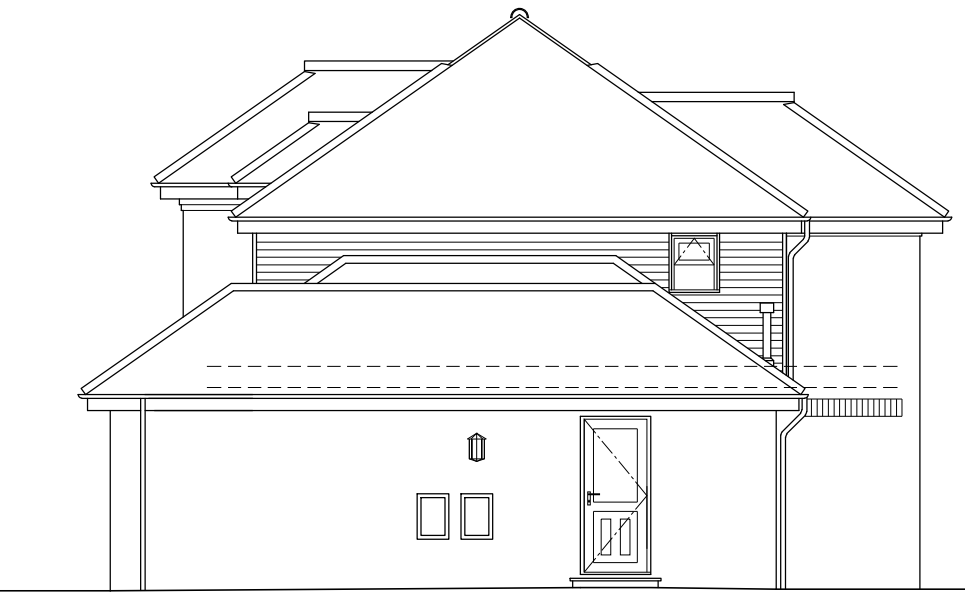
AS EXISTING EAST ELEVATION
