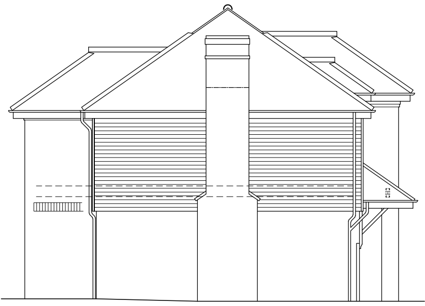
AS EXISTING WEST ELEVATION
