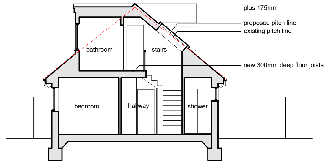
proposed section south-north
