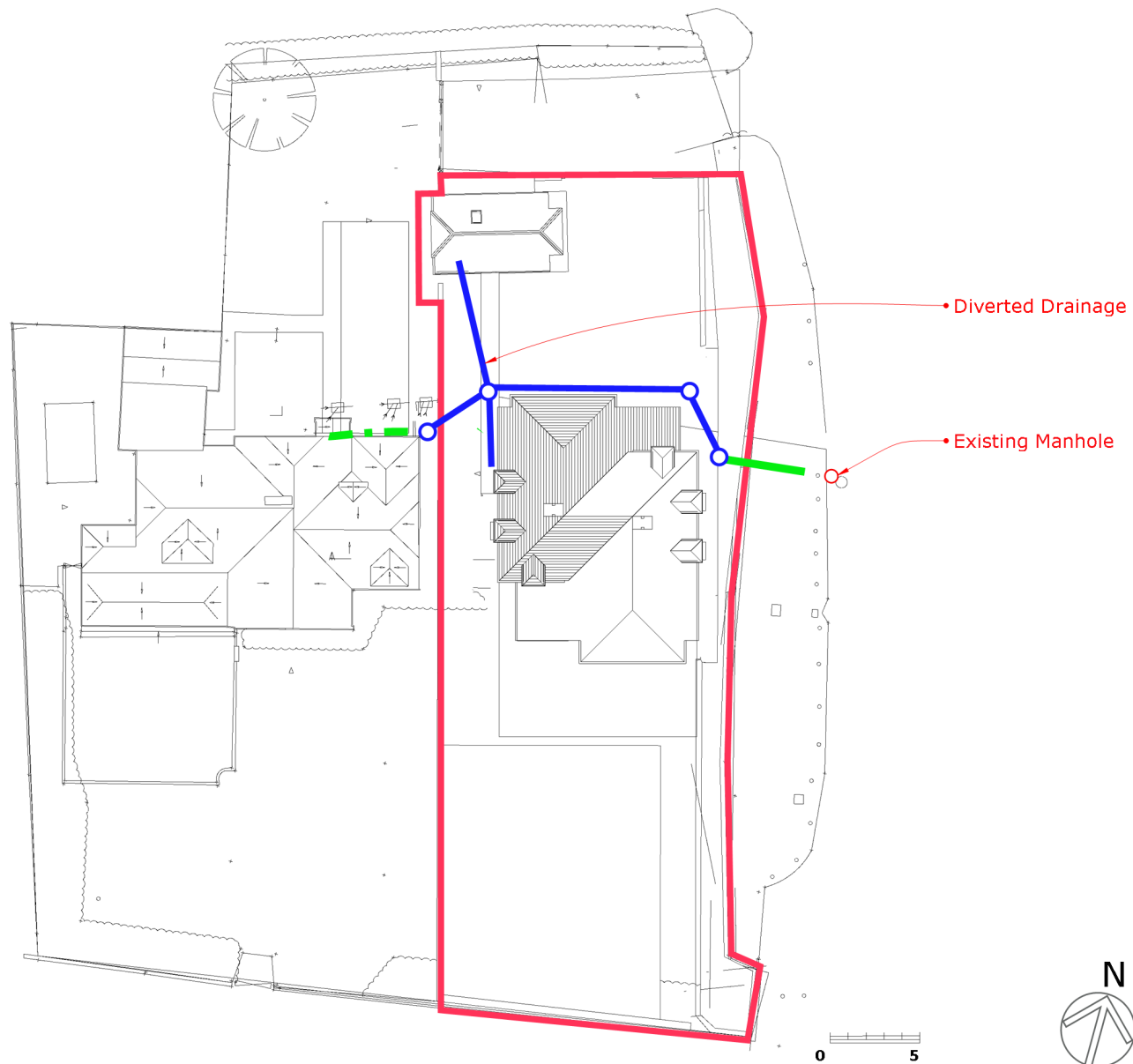
Drainage diversions 1:250 @a3 (Indicative)
