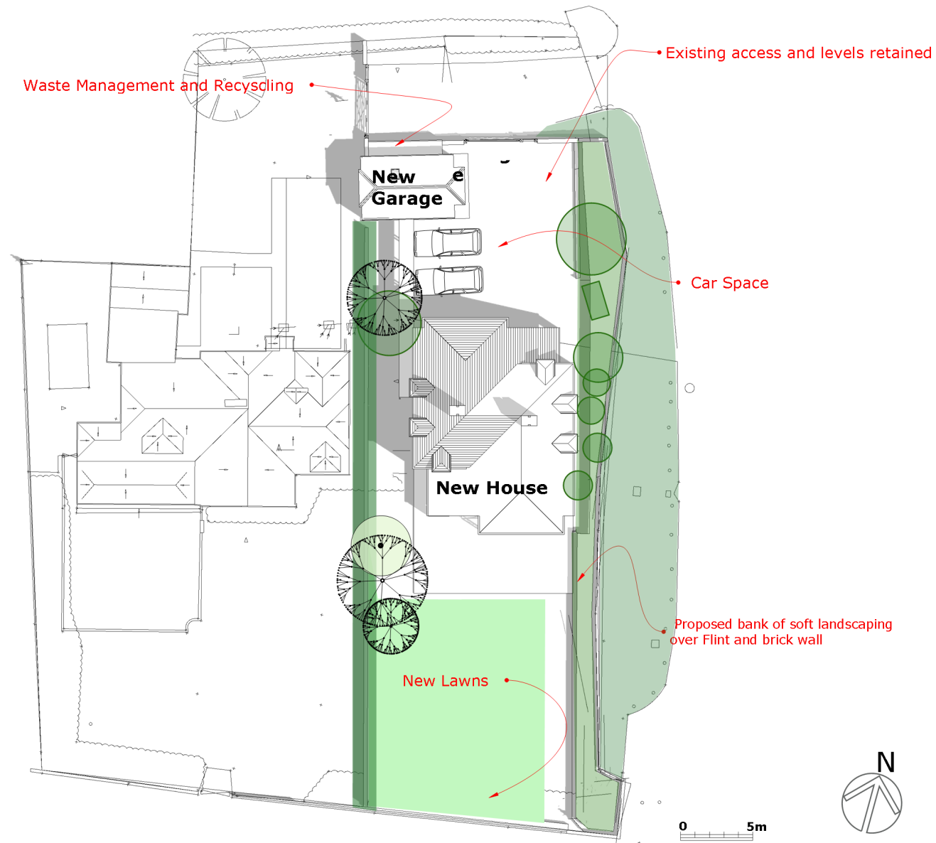
Proposed Landscaping and Car Parking 1:250
