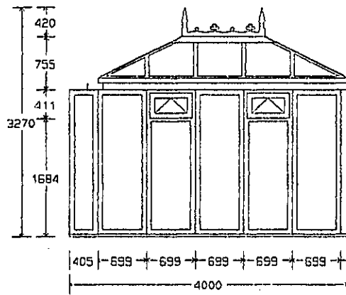
LEFT ELEVATION
