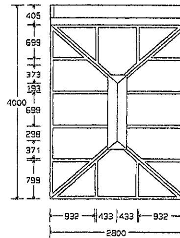
ROOF
