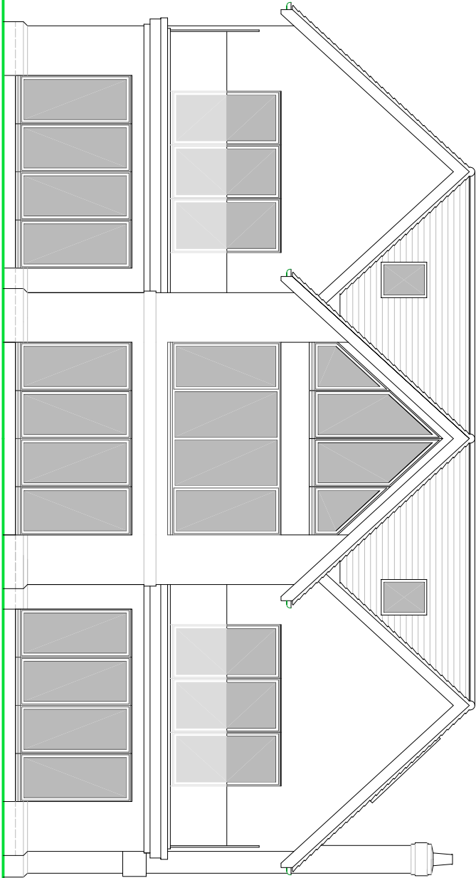
SOUTH ELEVATION
