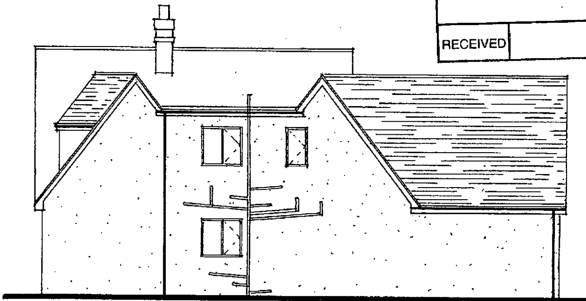
East Elevation - as proposed
