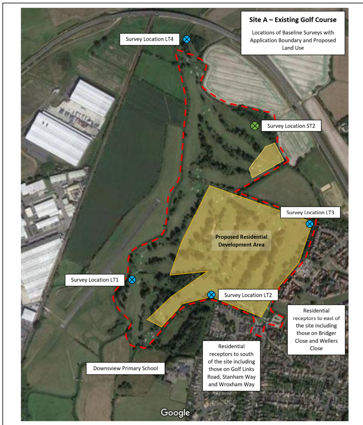
Figure 1: Noise Monitoring Locations at Site A
