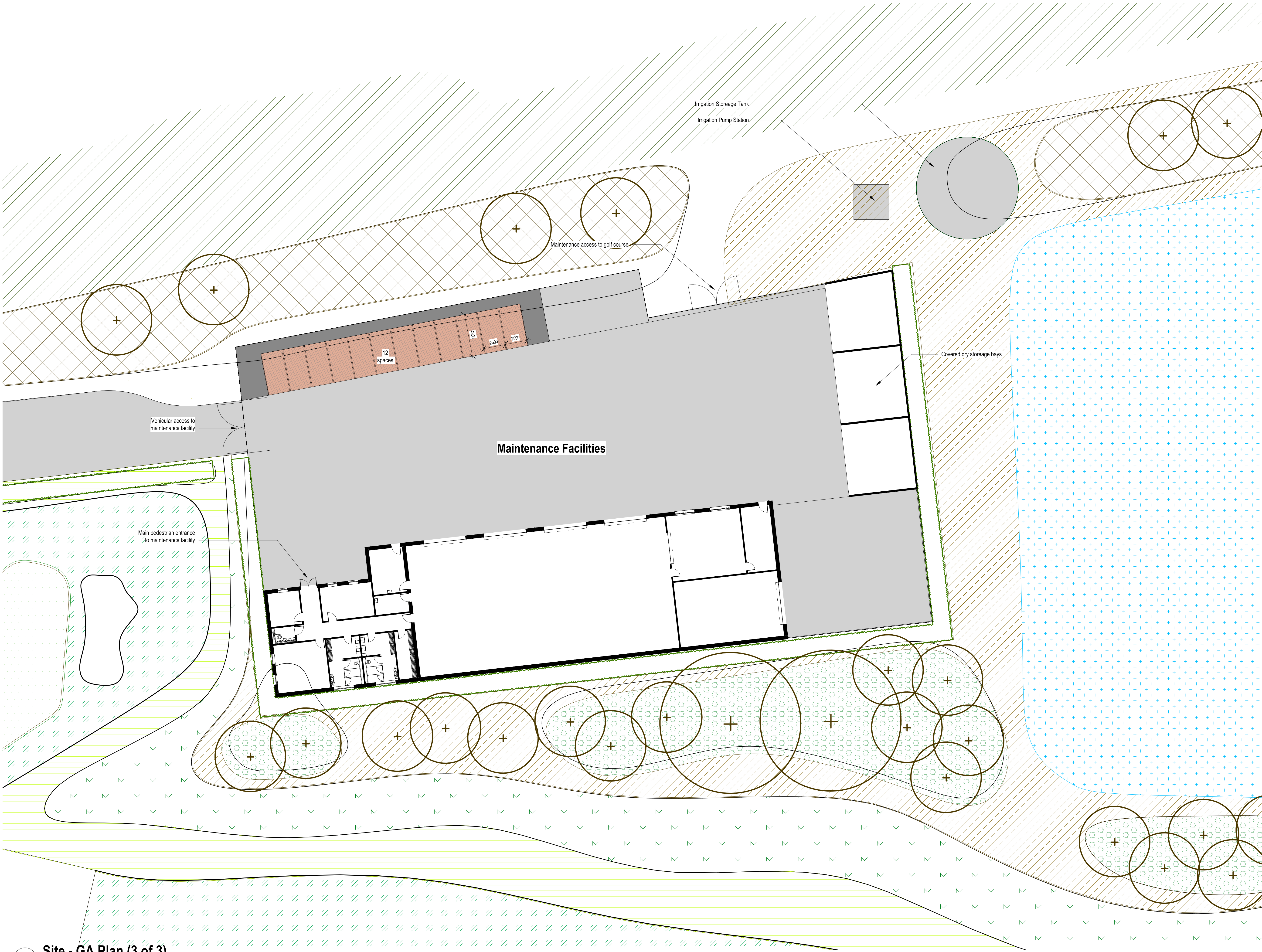
1 Site - GA Plan (3 of 3) 1 : 200
